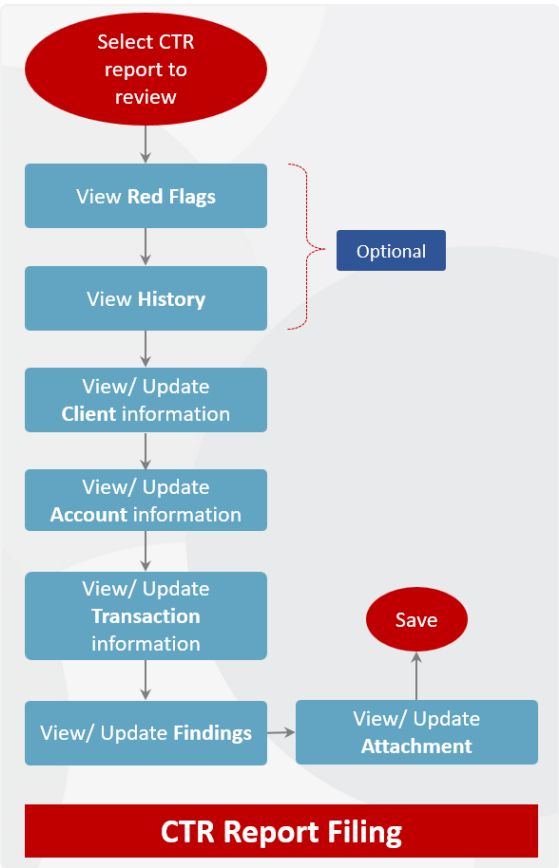
Figure 1.0: Apps Process Flow for CTR Report Filing
