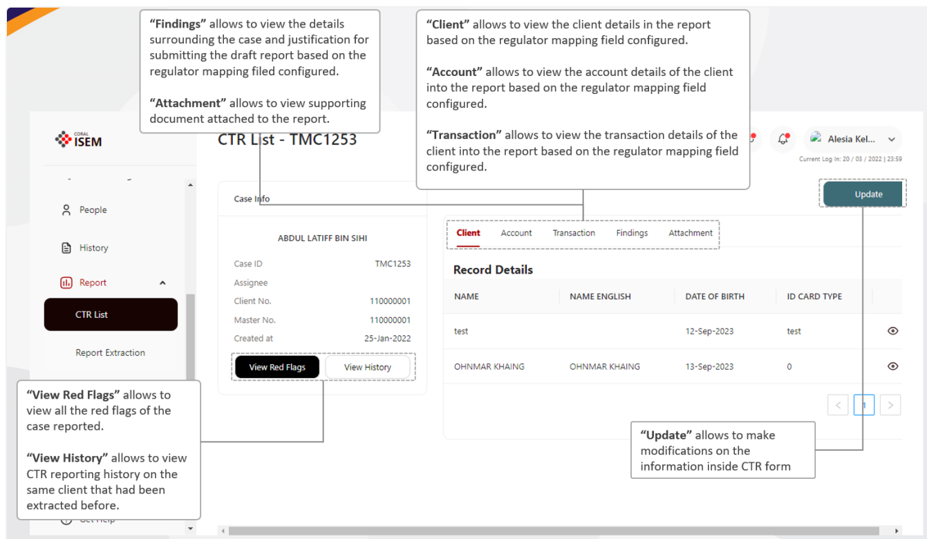
Figure 2.2: CTR List Details
